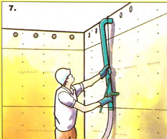
7. Provide fill holes at the top of the sheet and fill the wall cavity with the special lightweight concrete mix.
