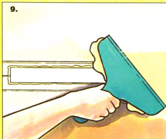
9. Apply HardiStop™ Base Coat and reinforcing tape to recessed and butt joints, internal and external corners as per James Hardie's jointing recommendations.
