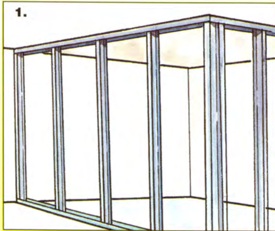
1. Fix steel top and bottom tracks to ceiling and floor and install the light gauge steel stud framing.
