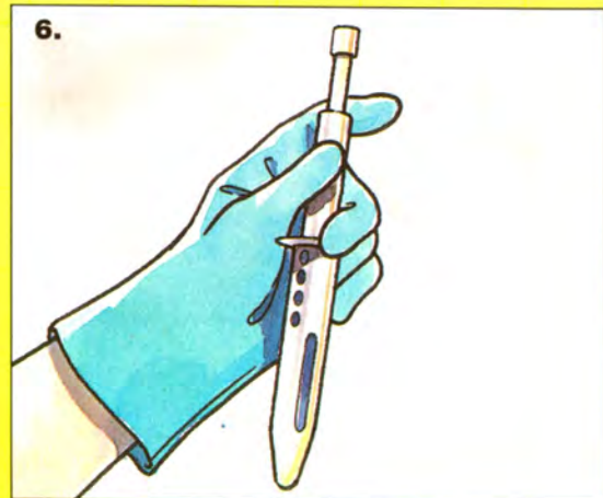
6. Check the mix consistency with the HardiFlow™ Meter to ensure optimum pumping performance. Then pump the mix to each floor.
