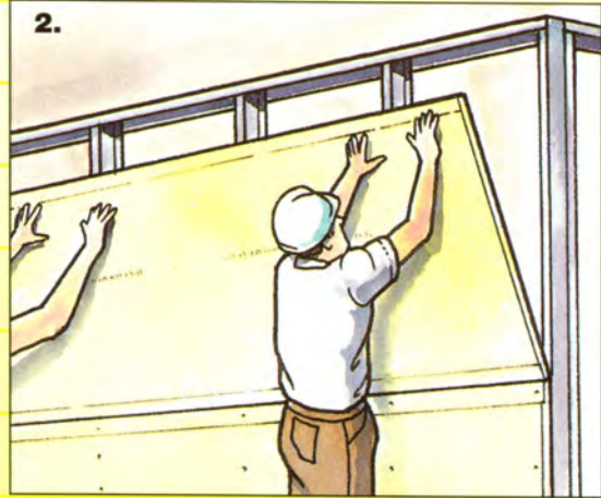
2. Attach HardiWall™ Sheets to one side of the frame using appropriate HardiDrive™ Fixings.
