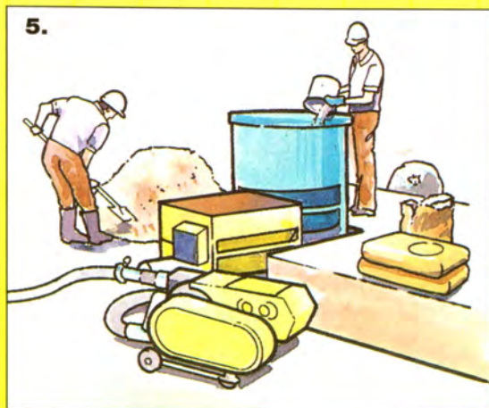
5. Prepare the core mix using HardiAdd™ Core Mix Additive with the specified mix ingredients at the designated mixing station.
